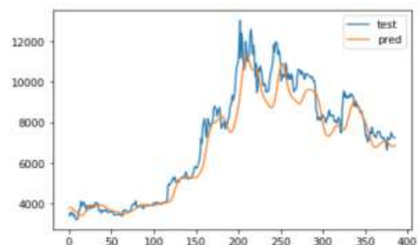
Fig.4.4. Data Visualization.
