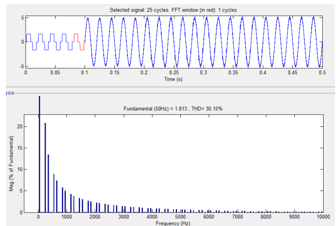
Fig.6.3. source voltage and current.
