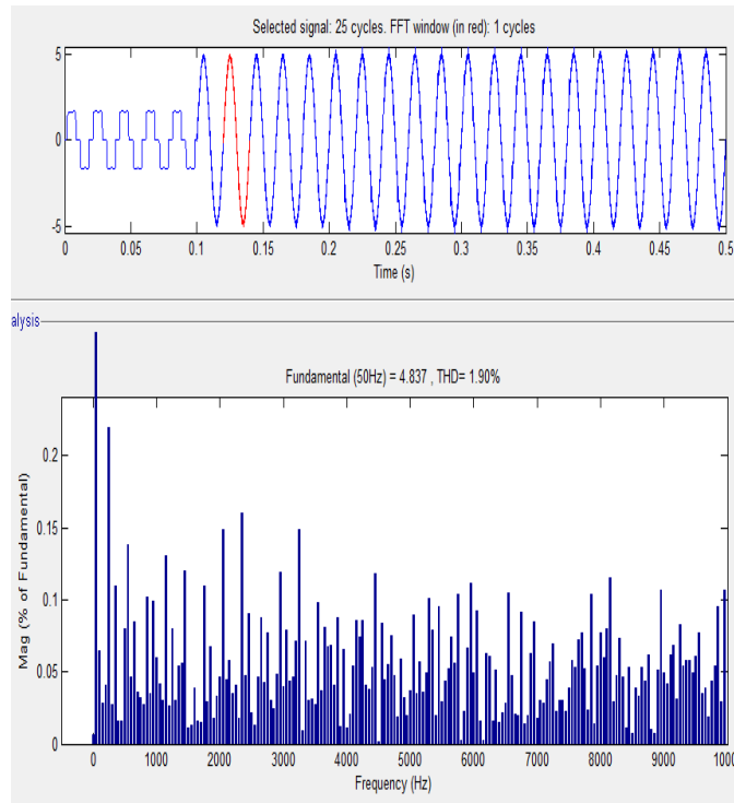
Fig.6.5 THD of source current after compensation.
