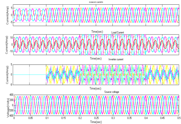
Fig.6.7. Simulation results of unbalanced Non-linear Load Source current, Load current, Inverter current and source voltage.
