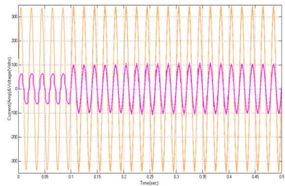
Fig.6.8 source voltage and current.
