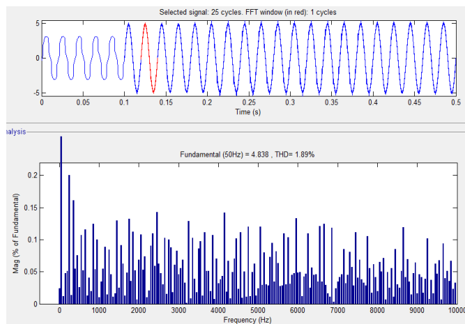
Fig.6.10 THD of source current after compensation.
