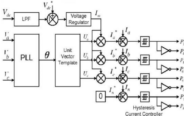
Fig.3. Block diagram of grid interfacing inverter control.
