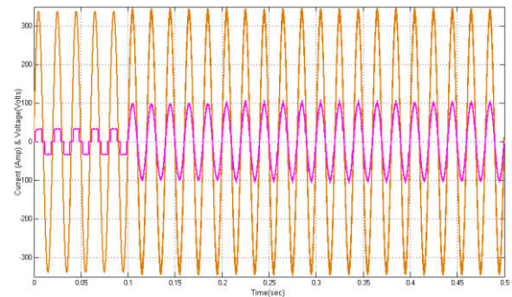
Fig.6.3. source voltage and current.
