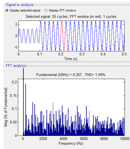
Fig.6.12 THD of source current of fuzzy controller
