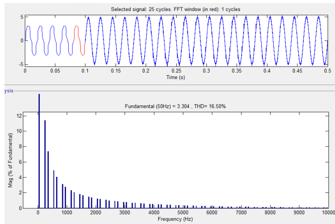
Fig.6.9 THD of source current before compensation.
