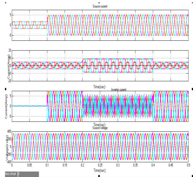
Fig.6.2. Simulation results of Balanced Non-linear Load Source current, Load current, Inverter current and source voltage.
