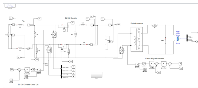
Fig.3.3. Simulation circuit.
