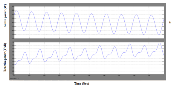
Fig.3.10. (a)Active power (b)Reactive power.
