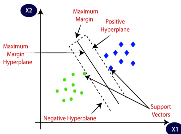
Figure 2: Analysis of SVM
