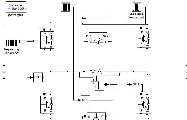
Fig.4.simulink circuit for 7 level inverter
