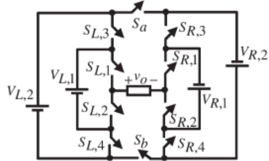
Fig.2. Proposed 31-level inverter.
