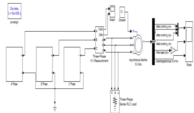
Fig.8. Simulink circuit induction motor fed 31 level inverter
