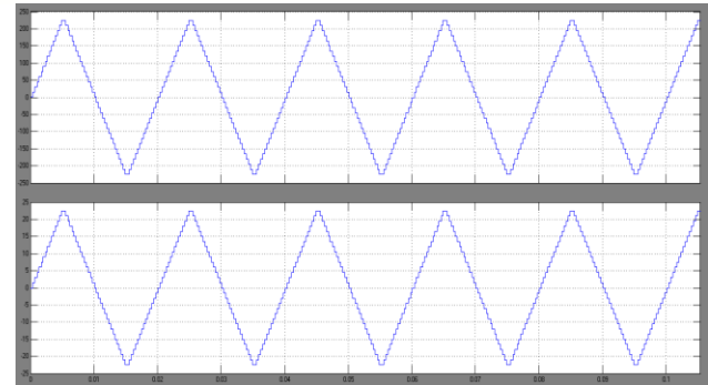
Fig.7.Simulation results voltage and current for 31 level inverter
